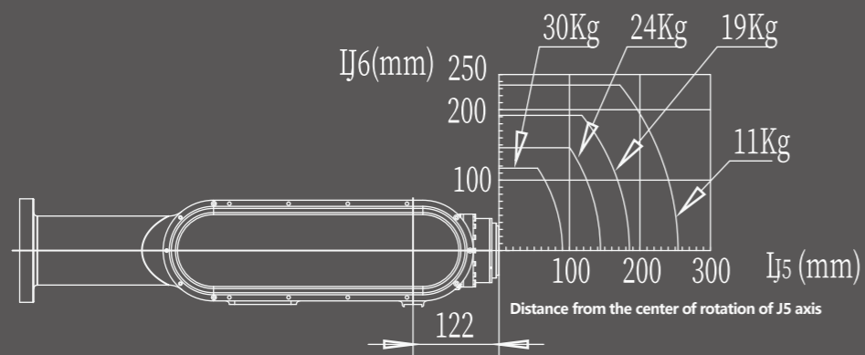
SF30 - C1850 Load Range Curve Chart
